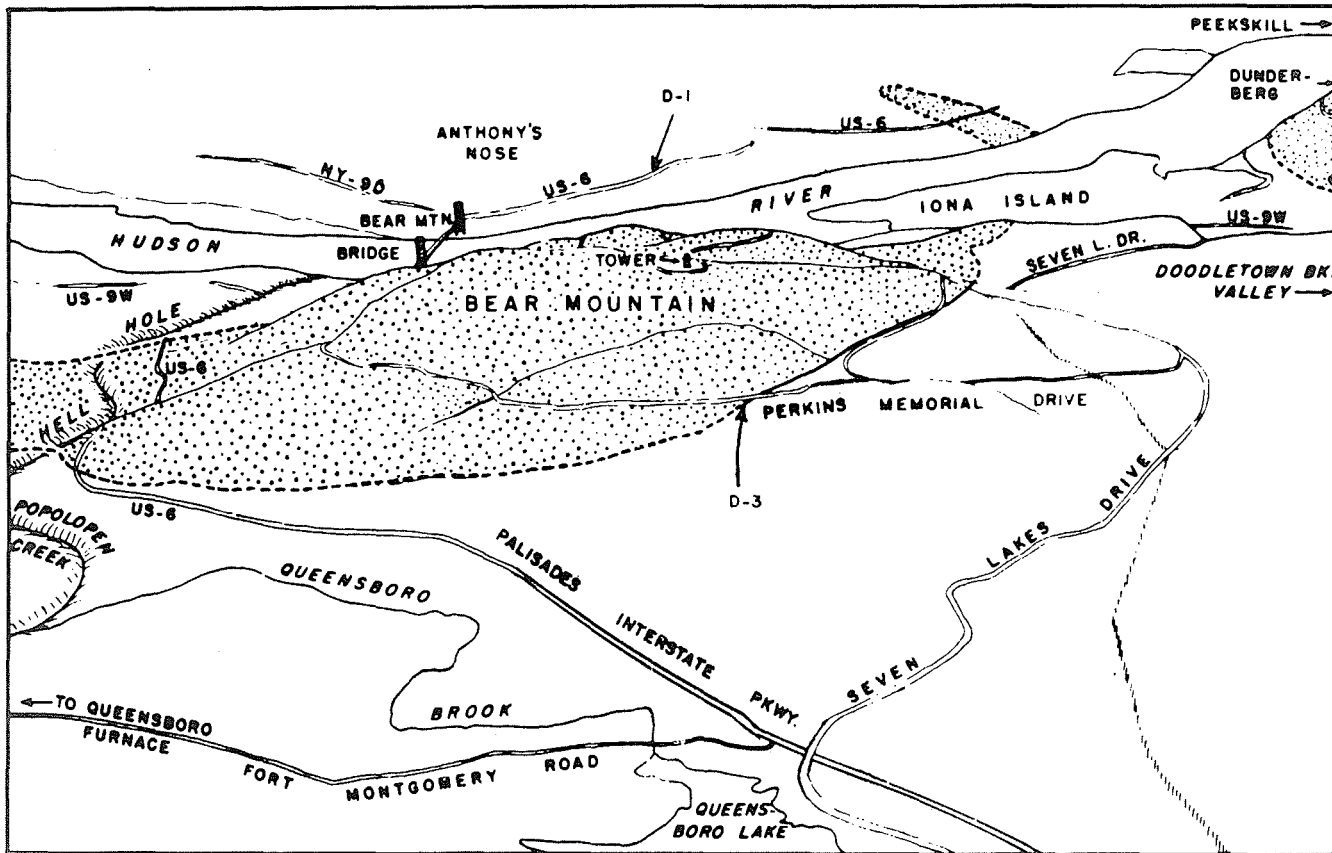
FIG. A VIEW OF BEAR MT., N.Y. LOOKING EAST FROM 5000 FT. STORM KING GRANITE STIPPLED
