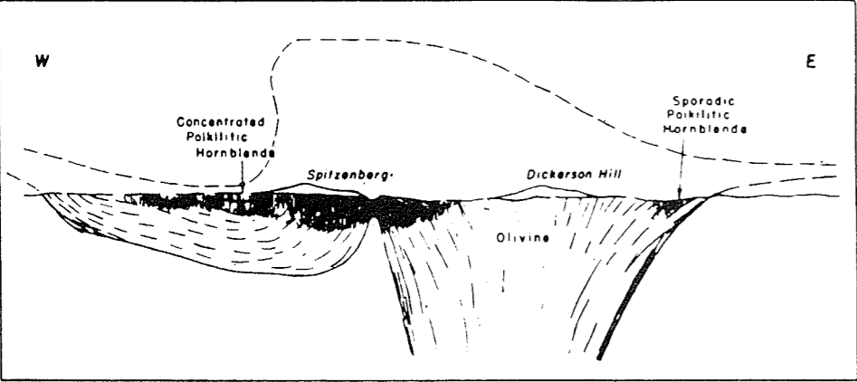
A possible interpretation of the subsurface extension of the Cortlandt complex. AFTER BUCHER (1948)
